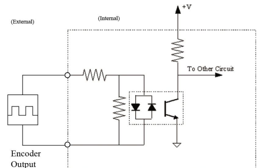
DC INPUT (Source) for Control Signals
