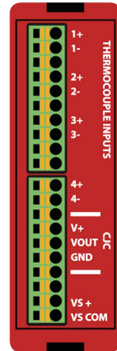
EZRPL-IO-4THIE
